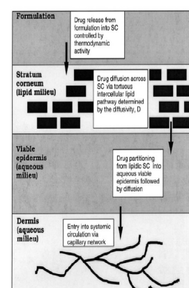
Fig. 1. Schematic representation of the transport processes involved from the release of the drug from the formulation to its eventual uptake by the dermal capillaries.
